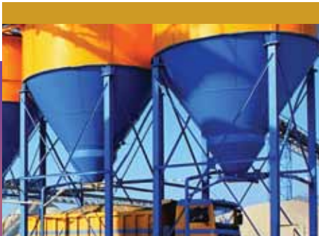
Load cells and weighing systems transform standard silos into scales for inventory or true weight detection
